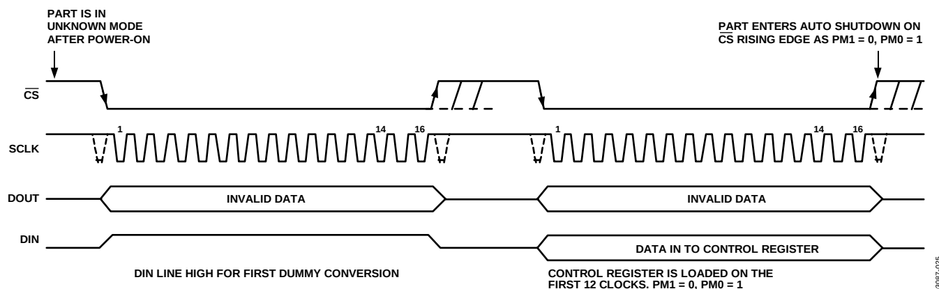
Figure 25. Placing the AD7904/AD7914/AD7924 into Auto Shutdown Mode After Supplies Are First Applied
