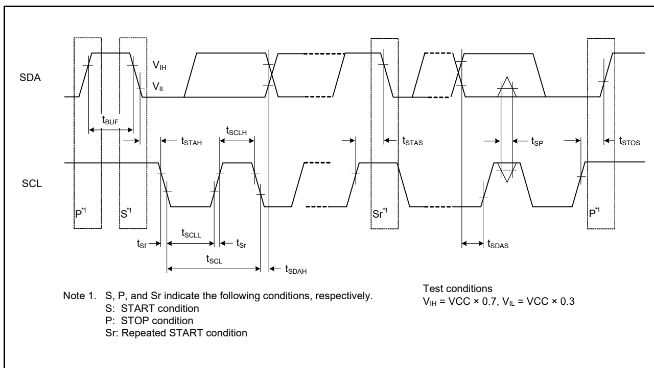
Figure 5.52 IIC Bus Interface Input/Output Timing and Simple I2C Bus Interface Input/Output Timing
